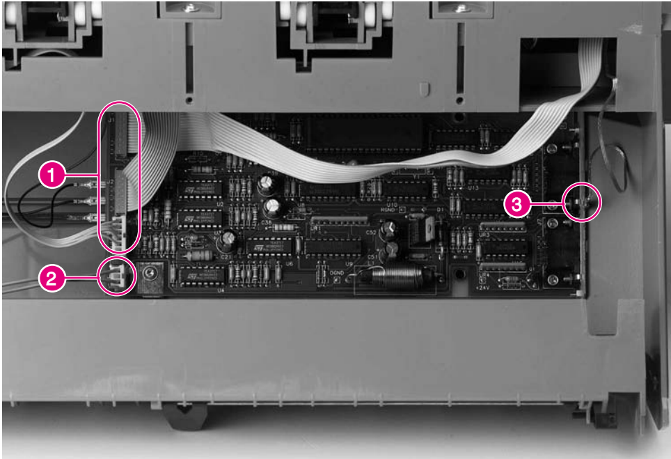
Figure 6-185 Stapler Controller PCA (2 of 3)
