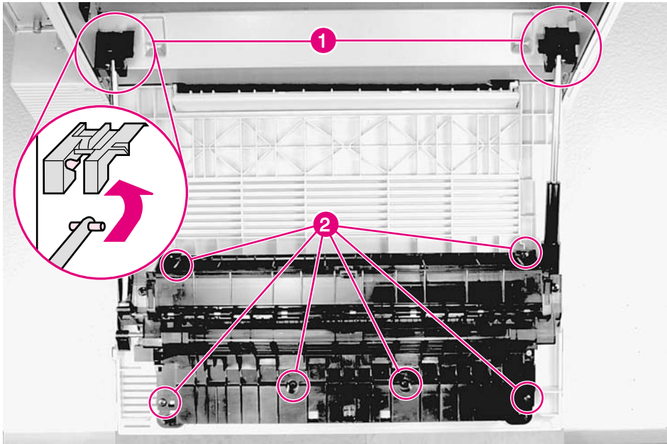
Figure 6-14 Diverter Assembly
