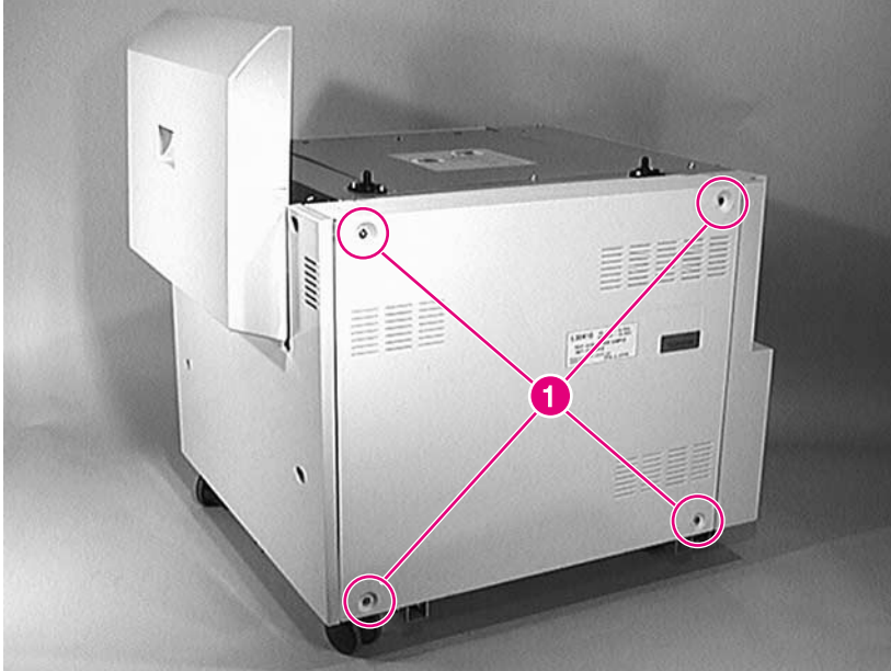
Figure 6-84 Back Cover
