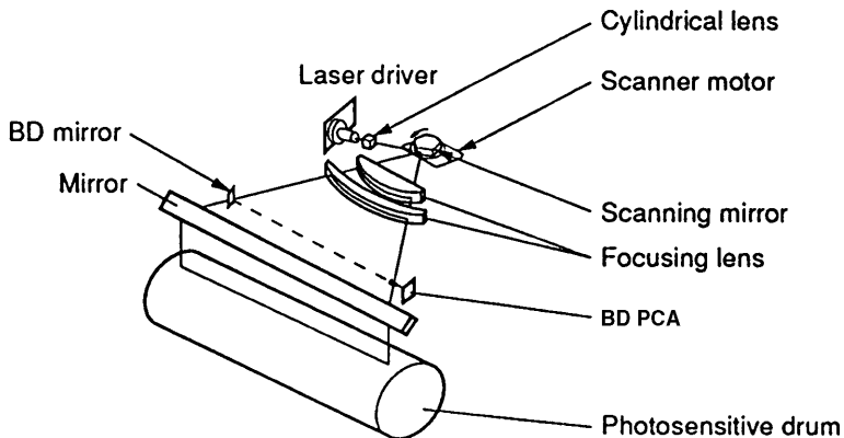
Figure 5-10 Image Writing
