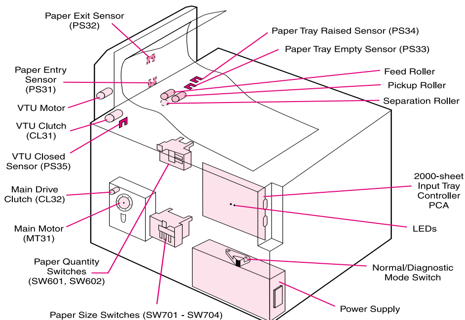
Figure 5-17 2000-sheet Input Tray Sensors, Switches, Clutches, and Motors
