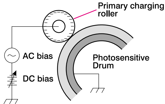
Figure 5-9 Primary Charging Roller
