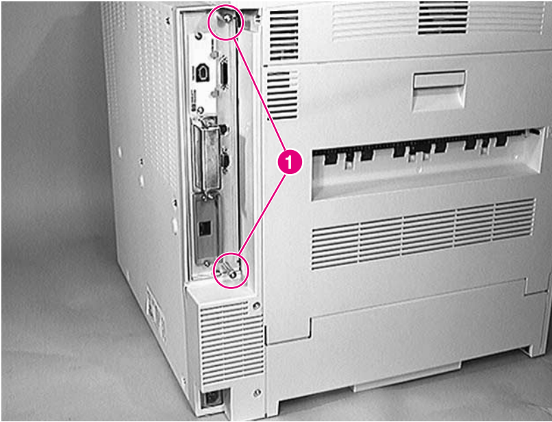
Figure 6-35 Formatter Assembly
