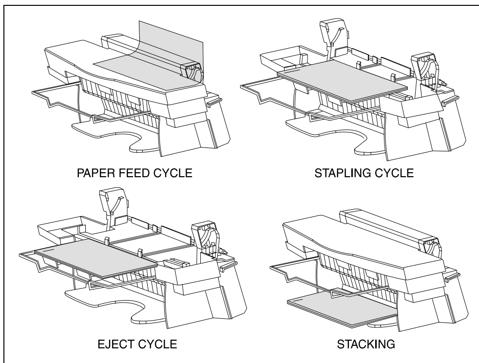
Figure 5-27 Stapler Cycles
